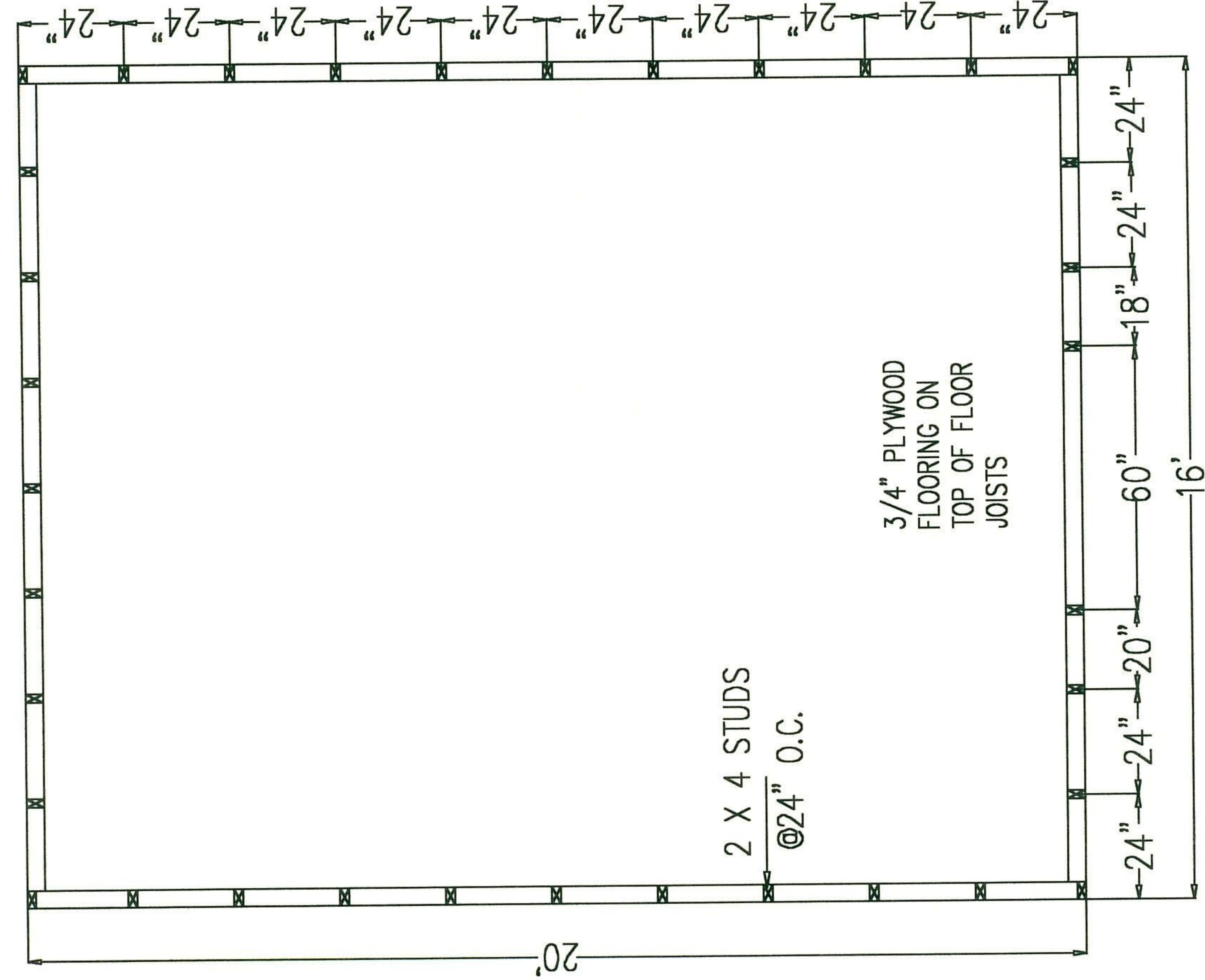
FLOOR PLAN
